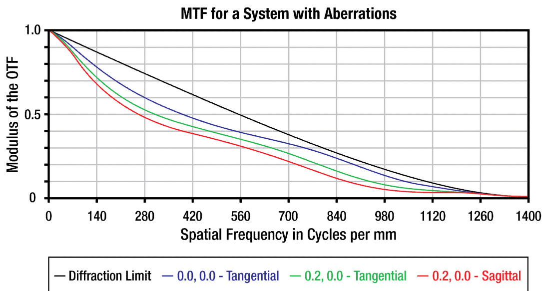
Figure 26: MTF for a system with aberrations. The upper traces are the diffraction limited MTF; the lower traces are actual performance due to geometric aberrations (mostly field curvature). Note that the MTF (the modulus of the Optical Transfer Function, or OTF) is worse than the diffraction limit on-axis (difference between black and blue lines) and falls off further at larger field radii (green lines). Curves were obtained using Zemax ray-tracing software.
