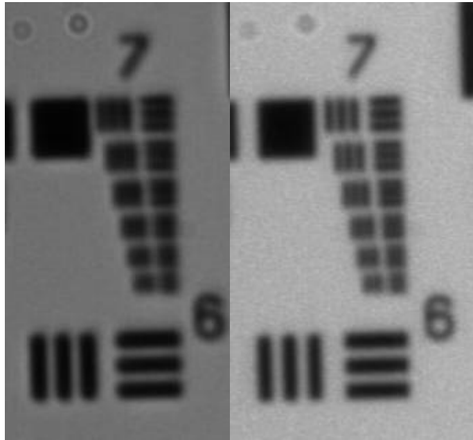
Figure 3: Condenser aperture closed (left) and wide open (right); note increase in resolution by \sim 2 elements. Exact improvement depends on both objective and condenser NA.
