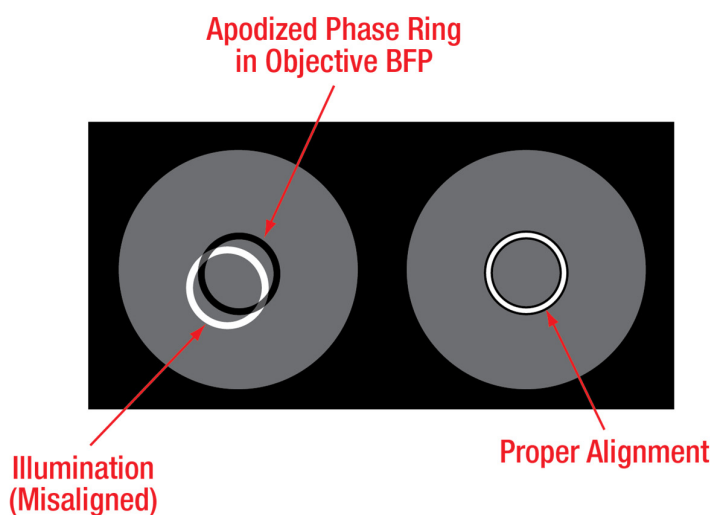
Figure 13: Aligning phase rings: when looking at the objective BFP, the annular illumination must fall on top of the darker apodized phase ring in the objective, or else contrast will be effectively brightfield instead of phase.
