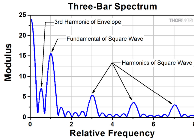
Figure 27: Spatial frequency content of USAF 3-bar target.
