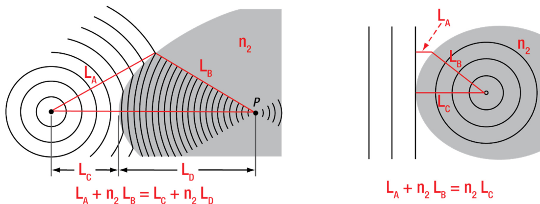
Figure 12: Equal time paths, defining the correct curved surface to form an image. Note that the formula (and hence the curve shape) for imaging one point to another (Left) is different than for focusing a plane wave down to a point (Right).
