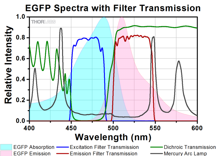
Figure 11: Spectra of an Hg arc lamp (gray), the EGFP fluorescent protein (light blue: absorption; pink: emission) and a filter set designed for EGFP (blue: excitation; green: dichroic; red: emission). Notice the general lack of lamp power in the excitation band – one reason Hg lamps are not so good for EGFP. Also note the strong lamp band at 546 nm; if one was really worried about filter leakage, one would trade off light collection to narrow the emission filter to cut that line out. The blue (~400 nm) transmission of the dichroic does not matter, since the excitation filter will have already removed that energy from the light beam. Just in case, though, the emission filter blocks at those wavelengths.
