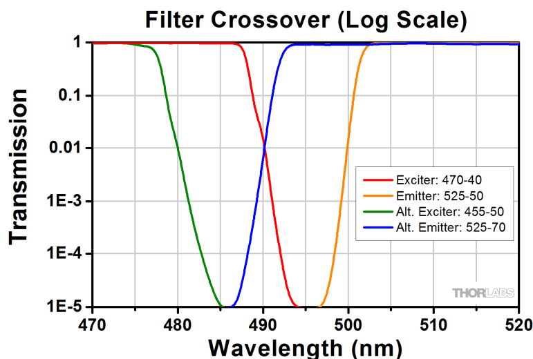
Figure 14: Filter crossover, log scale. Note that either set of filters crosses at OD > 5, for a combined OD > 10 at crossover (since transmissions multiply, \log(T) – i.e., ODs – add). This is excessive; in the emission filter transmission band, OD is ~5 from the excitation filter, and vice-versa, so there is little point in having higher OD over a few nm of bandwidth near crossover. Having the filters cross at OD 3+ gives OD 6+ blocking through the entire band, and allows the filter transitions to be brought closer together so that you can catch more of the emission light. Typically ~ 10 - 15 nm between the excitation filter cut-off to the emission filter cut-on is fine.
