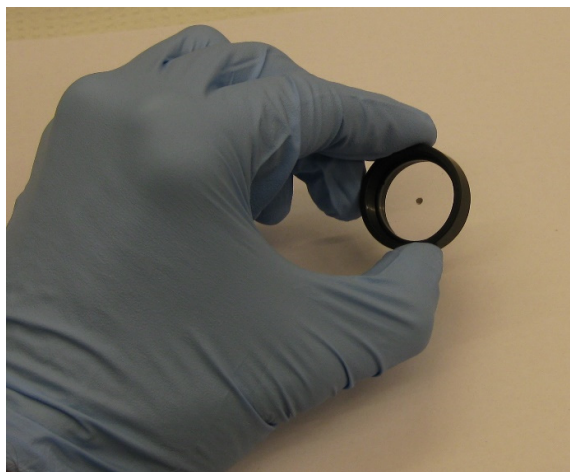
Figure 1: Home-Made Phase Mask: 1.25 mm diameter stearin candle soot spot, with transmission \sim 10\% , on a coverslip mounted in an SM1 tube.
