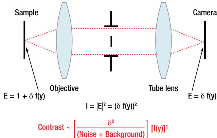
Figure 10: Darkfield: Contrast enhanced by 1 / \alpha , i.e., 1 / (\text{attenuation of the main illumination}) ; darkfield uses \alpha \sim 0 , so in theory contrast approaches \frac{1}{0} which goes to infinity. In reality, however, the background light limits how small the denominator can get.
