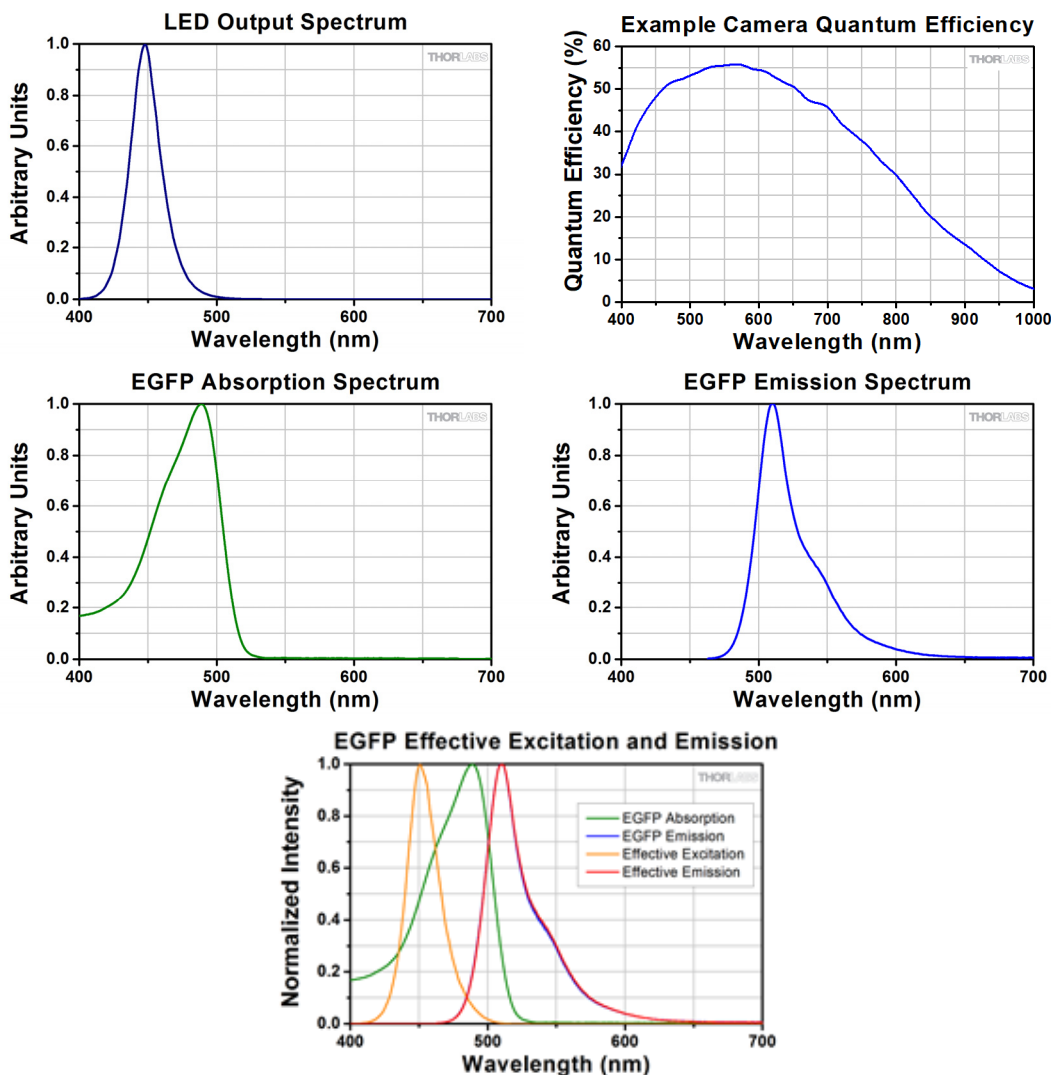
Figure 12: The effective excitation (orange line) and emission (red line) spectra are respectively the point-by-point products of the dye absorption and light source photon flux, and the dye emission and detector quantum efficiency. (Bottom): Note that the excitation (an LED, emitting in a narrow range around 450 nm) is not centered on the absorption maximum, and so the effective excitation is shifted substantially. The emission falls in a relatively flat area of the camera QE curve, and so it is not changed noticeably.
