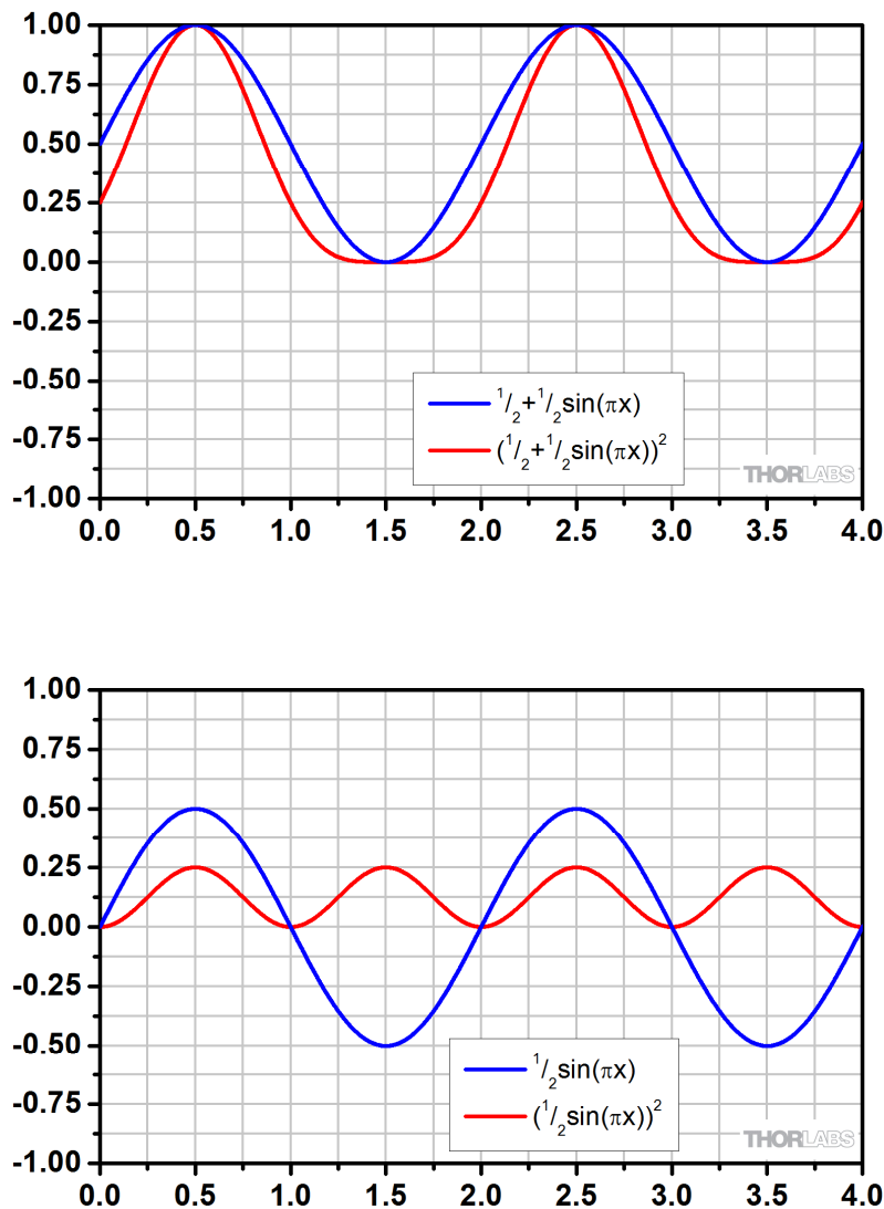
Figure 11: Effect of Squaring: The square of [\frac{1}{2} + \frac{1}{2}\sin(ax)] (Top, red trace) does not look like the square of [\frac{1}{2}\sin(ax)] (Bottom, red trace), even though both have the same initial amplitude (blue traces).
