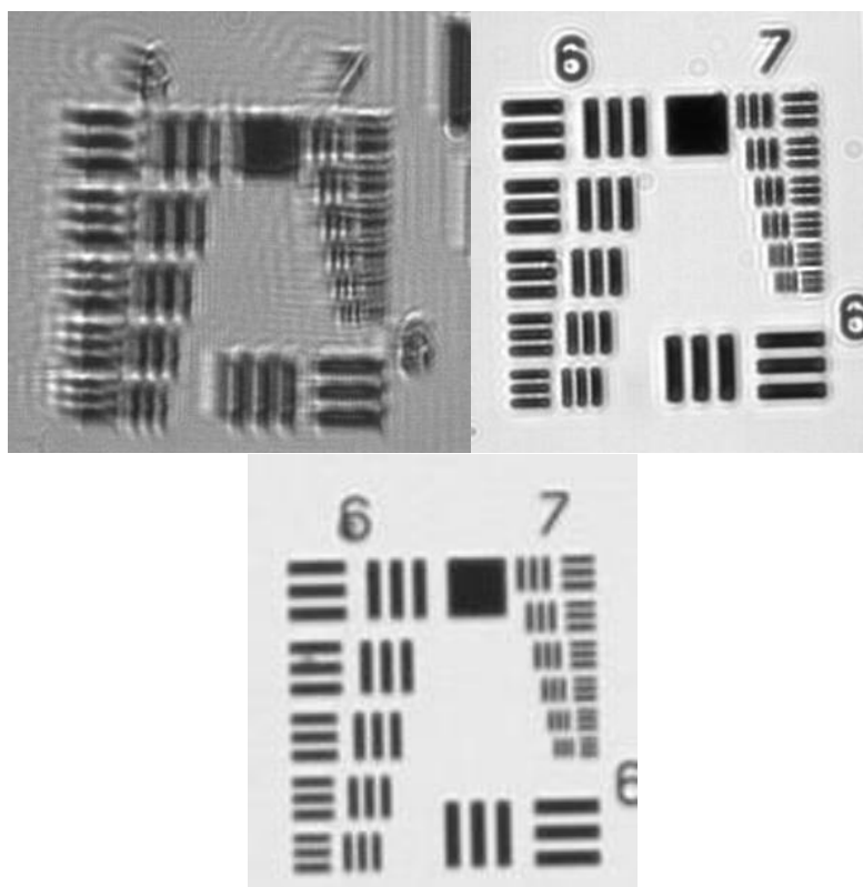
Figure 4: USAF target illuminated by an LED (upper left, NA \sim 0.003 ), a small condenser aperture (upper, right, NA \sim 0.01 ), and a diffuser (bottom, NA \sim 0.1 ). Note decreasing visibility of fringes.
