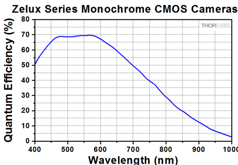
Figure 3: QE for a Thorlabs CS165MU(/M) camera (i.e., the fraction of incident photons at any given \lambda which are detected by the camera). For an inexpensive camera, this one is very good in the green. QE falls off toward zero as \lambda increases toward 1.1 \mu\text{m} , since the energy of a photon at that wavelength is below the 1.12 eV band-gap energy of the doped silicon. When the photon cannot excite an electron into an accessible state, it cannot be absorbed (and hence detected). For the same reason, silicon is transparent at \lambda > 1.1 \mu\text{m} .
