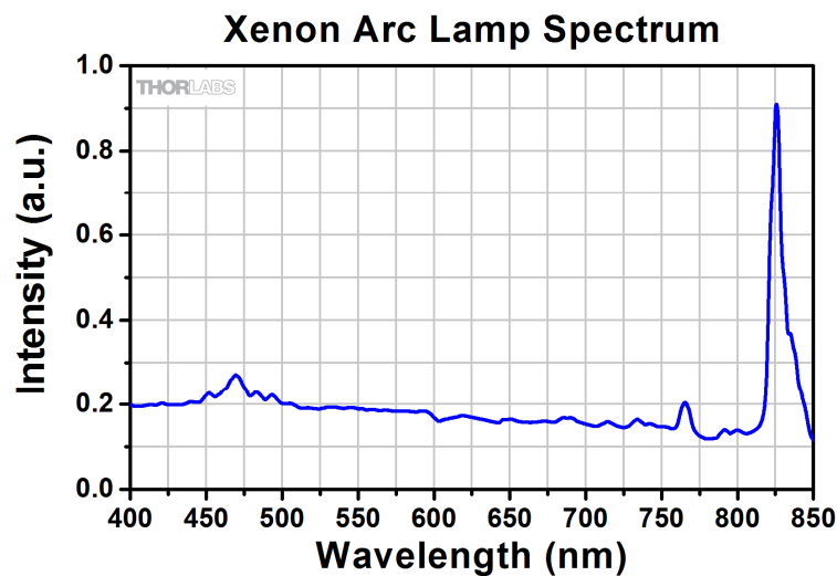
Figure 11: Xenon arc lamp spectrum (EXFO is the manufacturer). (Source: McNamara-Boswell Spectra Compilation)
