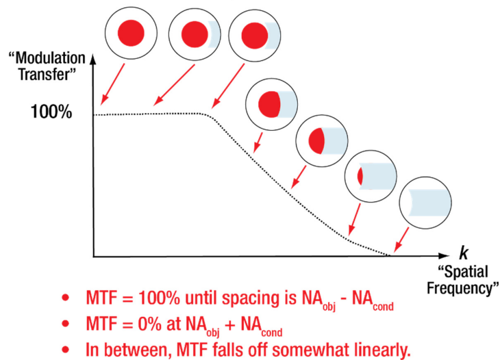
Figure 22: MTF for incoherent illumination, NA_{condenser} < NA_{objective}
