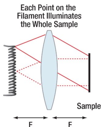
Figure 1: In Köhler illumination, each point on the filament illuminates the whole sample.
