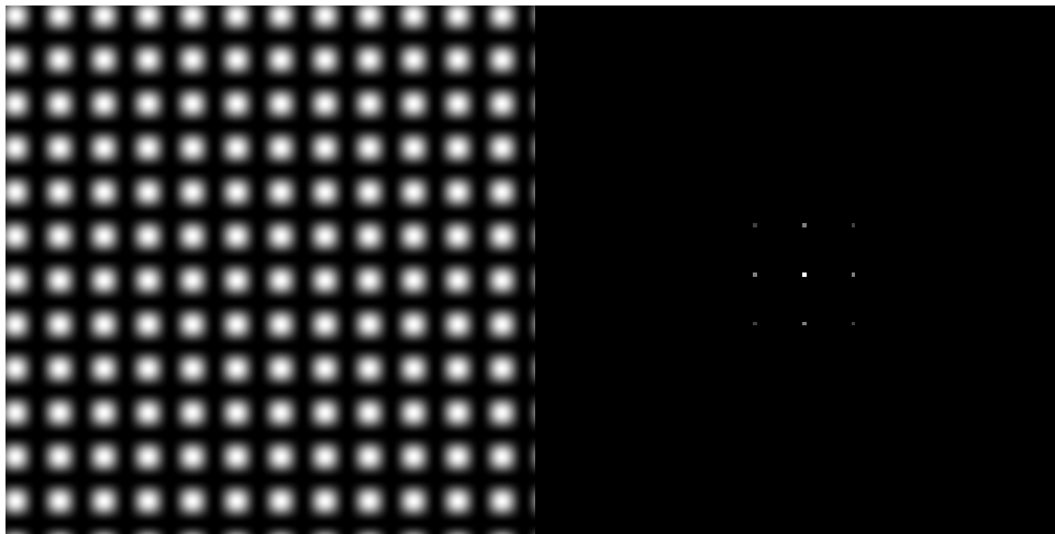
Figure 19: Multiplication of vertical and horizontal sine waves. Diffraction pattern is a “convolution” of Fig. 16 and Fig. 17 diffraction patterns.
