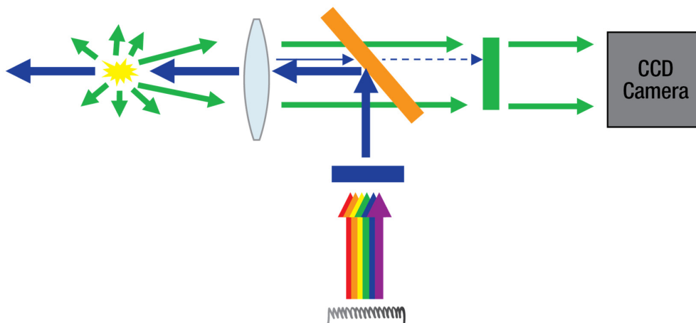
Figure 13: Epi-Fluorescence Geometry
