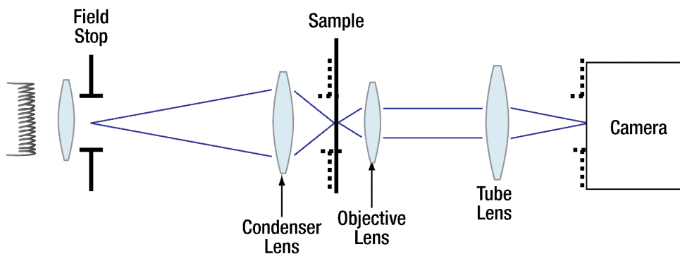
Figure 8: Conjugate planes:
