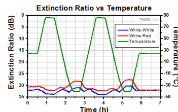
Click to Enlarge 7-hour temperature cycling test performed on a standard PN1550R5A1 PM fiber coupler shows that the PER measured for the white-white and white-red paths remains stable over a wide temperature range.
